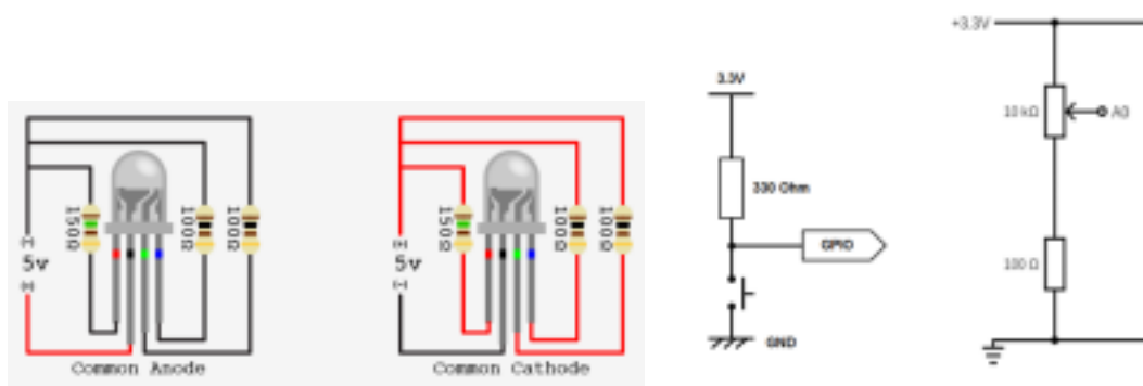
Figure 1.2 External Potentiometer Setup Figure 1.3 External Push
